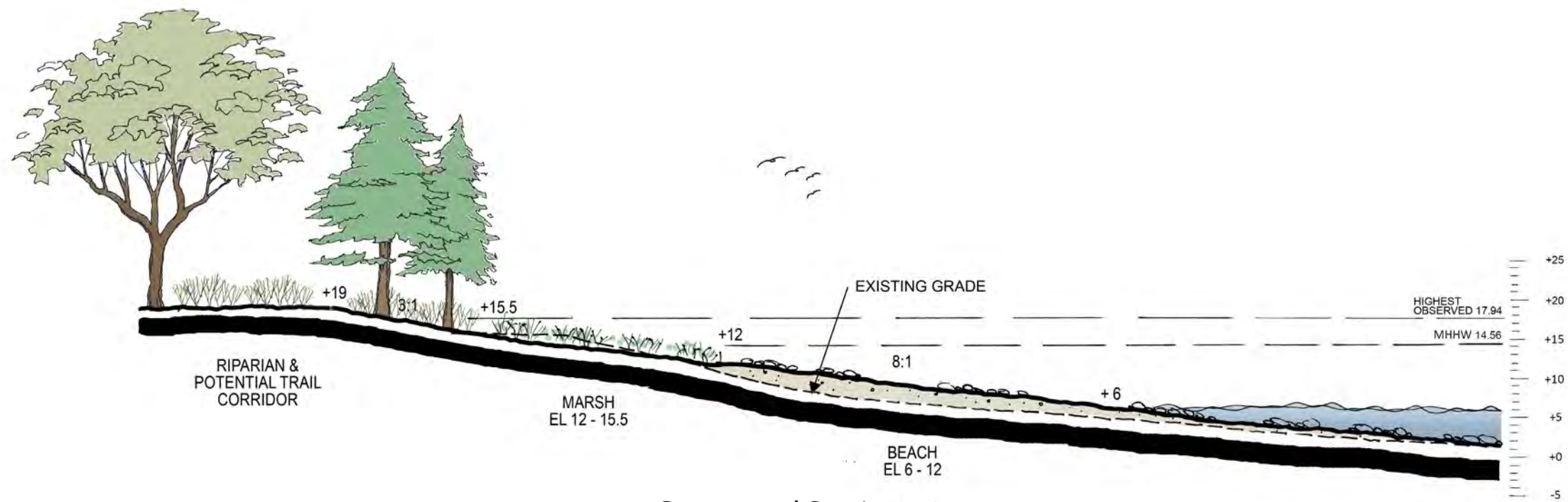
Conceptual Section 16
