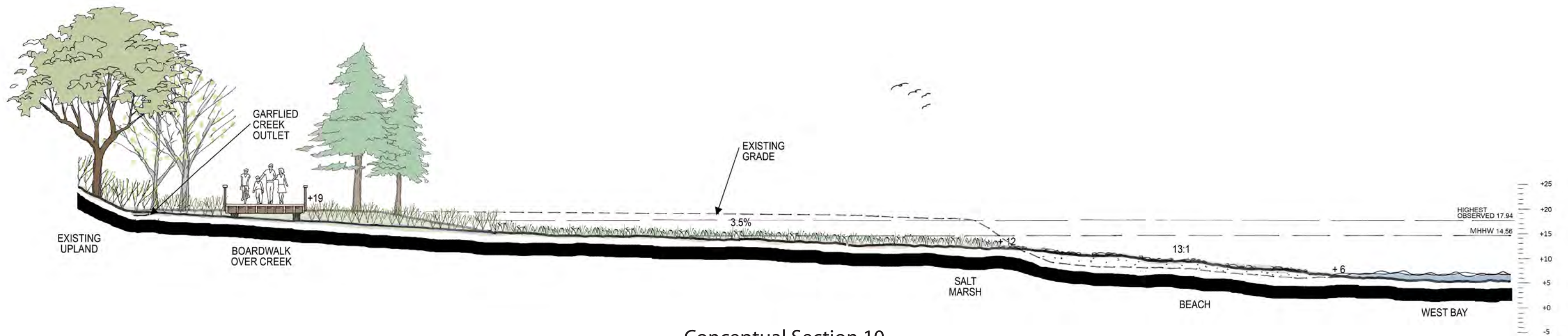
Conceptual Section 10
