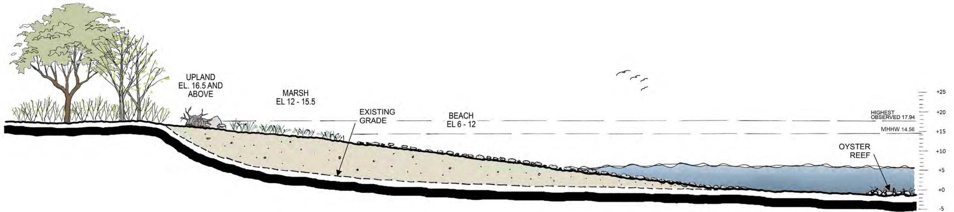
Conceptual Section 17
