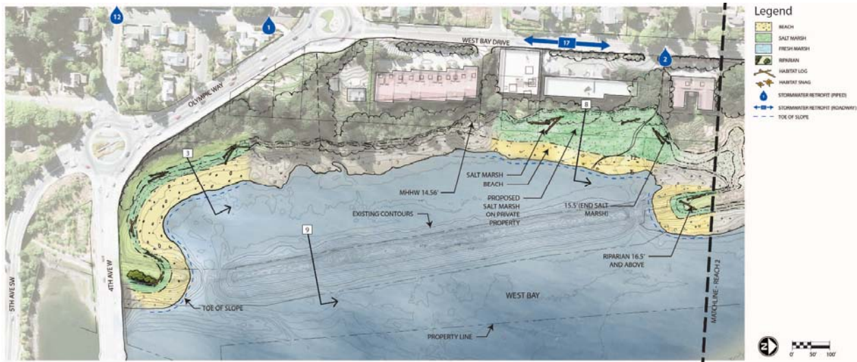
Figure 5. Lagoon Alternative 4.
