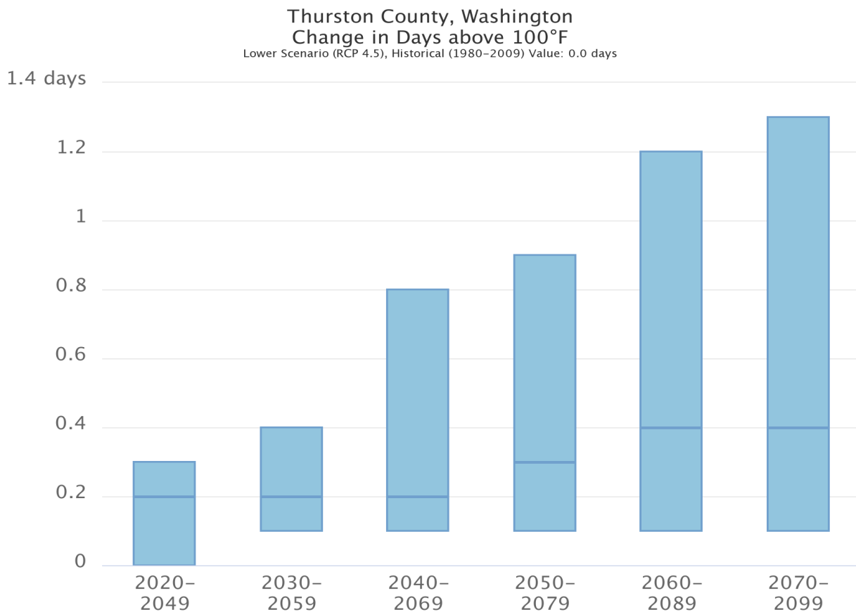
Figure A4. Change in the number of days per year with a maximum temperature > 100°F in Thurston County for future 30-year periods under RCP4.5 [15]. Change is in comparison to the historical baseline (1980–2009). The six blue bars show the 10th to 90th percentile range of projections; the dark blue line contained within each bar is the ensemble median.
