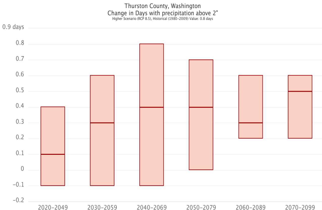
Figure A14. Change in the number of days when total precipitation is > 2 inches in Thurston County for future 30-year periods under RCP8.5 [15] . Change is in comparison to the historical baseline (1980–2009). The six red bars show the 10th to 90th percentile range of projections; the dark red line contained within each bar is the ensemble median.
