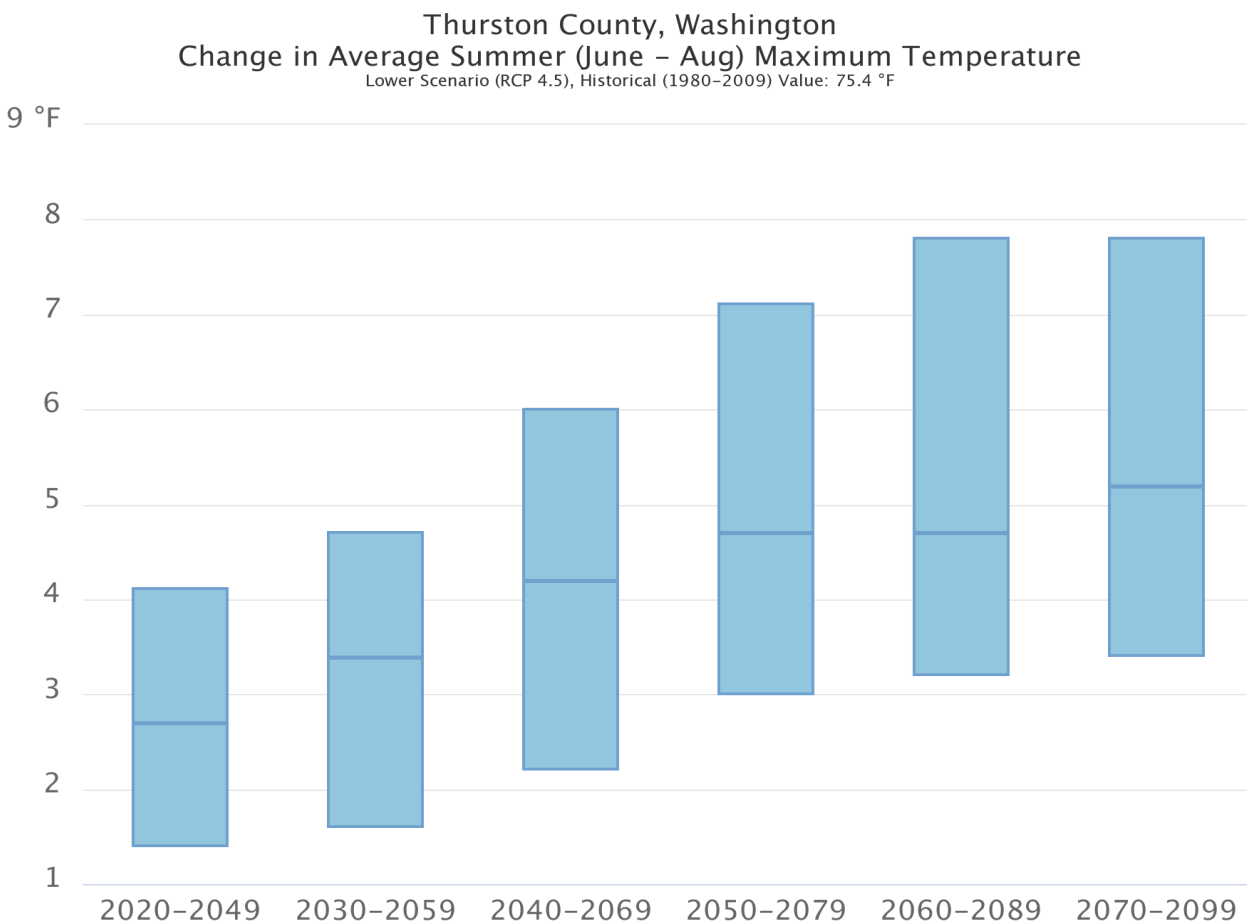
Figure A2. Change in the summer maximum temperature (°F) in Thurston County for future 30-year periods under RCP4.5 [15]. Change is in comparison to the historical baseline (1980–2009). The six blue bars show the 10th to 90th percentile range of projections; the dark blue line contained within each bar is the ensemble median.
