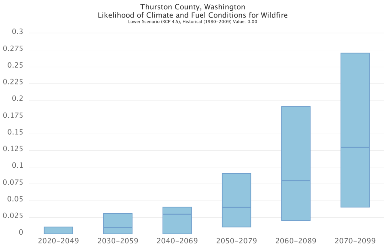
Figure A26. Likelihood of a year with climate and fuel conditions favorable for wildfire in Thurston County for future 30-year periods under RCP4.5 [15]. The six blue bars show the 10th to 90th percentile range of projections; the dark blue line contained within each bar is the ensemble median.
