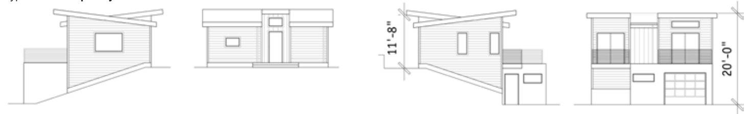
type G contemporary elevations:
