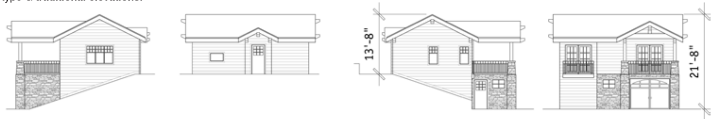
type G traditional elevations:
