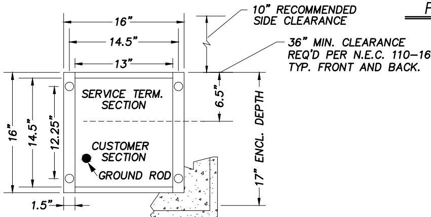
FLOOR PLAN
