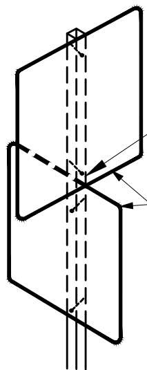
TRAFFIC CIRCLE SIGN MOUNTING DETAIL
