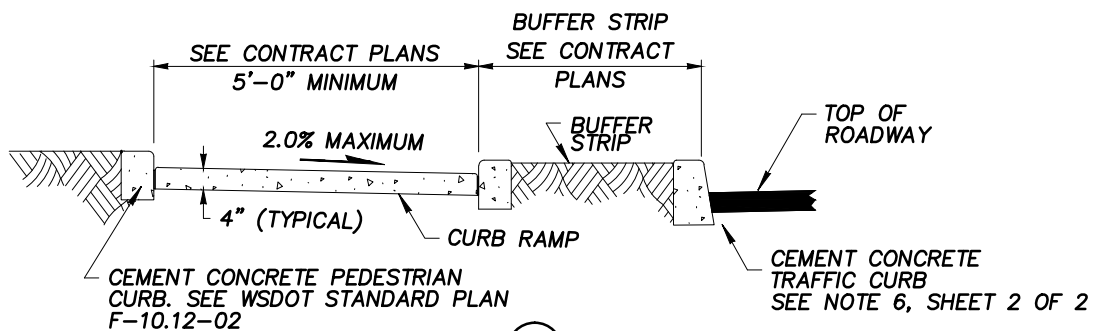
SECTION (B)
