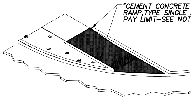
ISOMETRIC VIEW—TYPE SINGLE DIRECTION A
