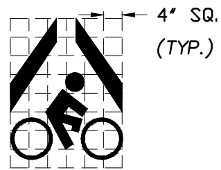
CYCLE DETECTOR SYMBOL
