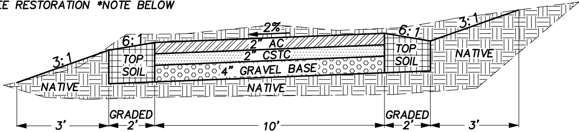
NEIGHBORHOOD CONNECTOR
