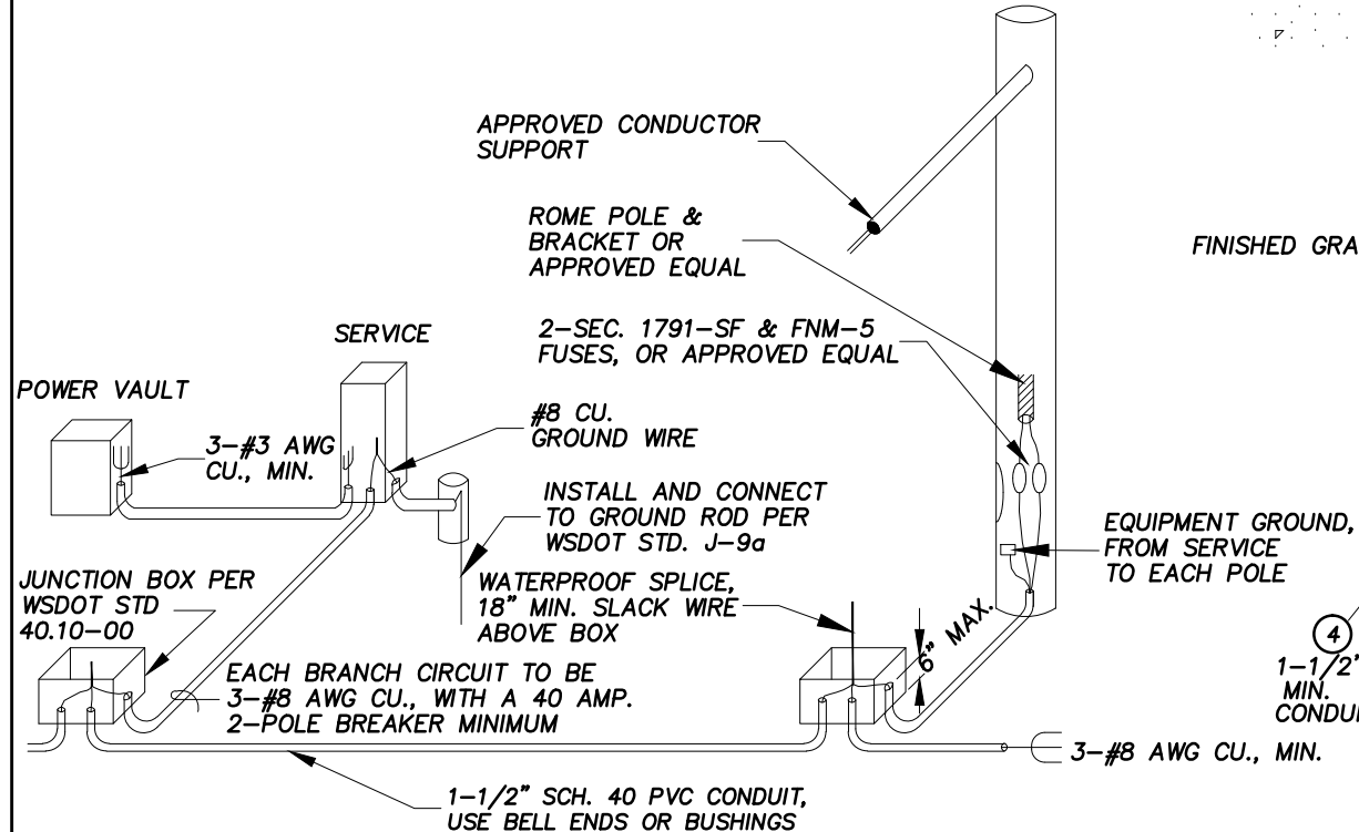
TYPICAL BASE DETAIL
