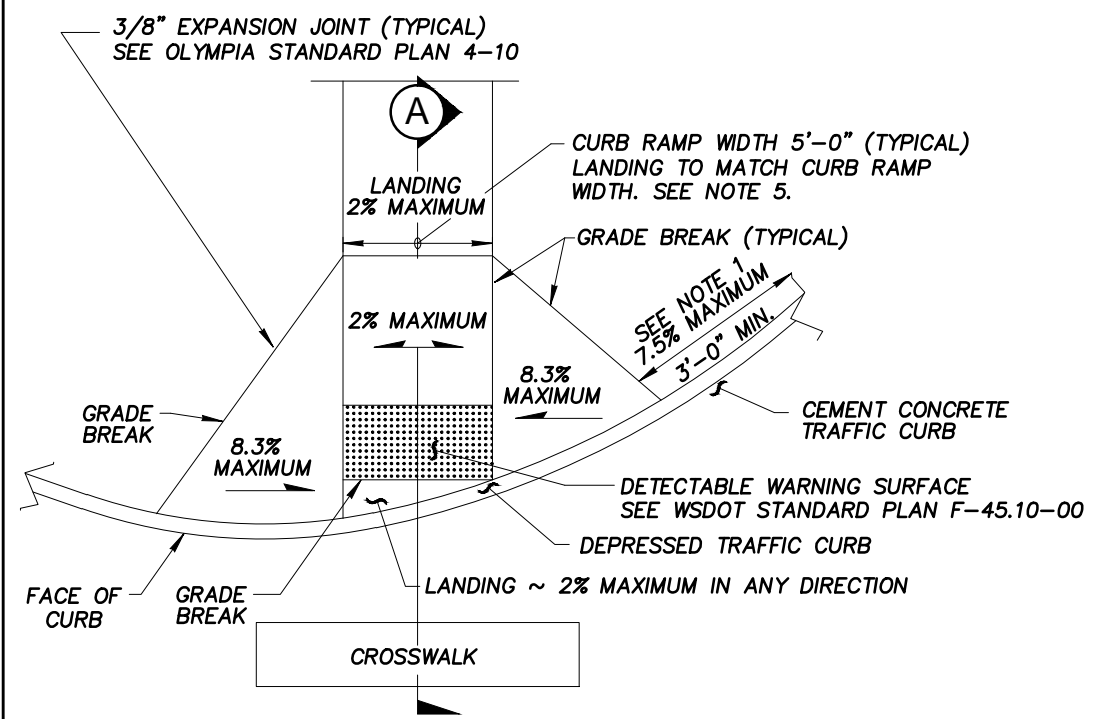
TYPE PERPENDICULAR C
