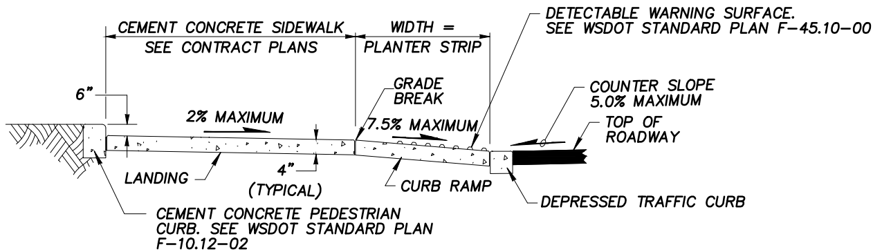
SECTION (A)
