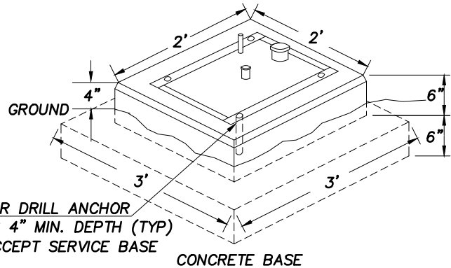
CONCRETE BASE
