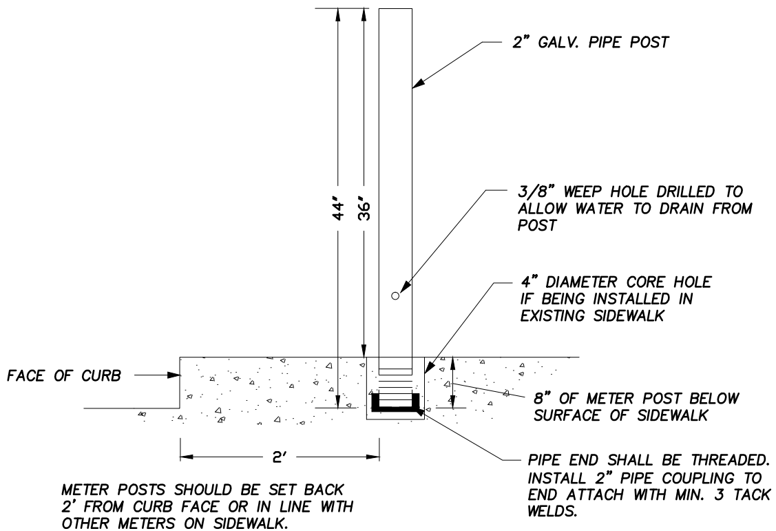
TYPICAL POST INSTALLATION IN EXISTING SIDEWALK AREA
