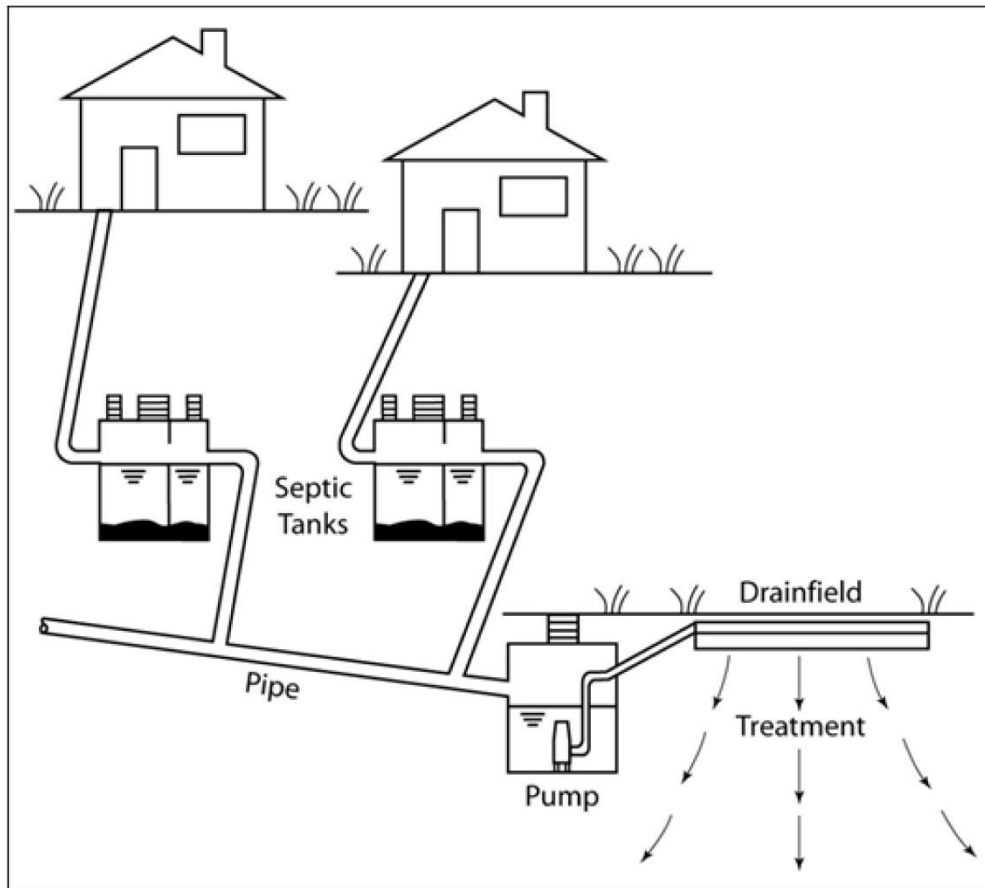
Figure 4.3 Community Onsite Sewage System
