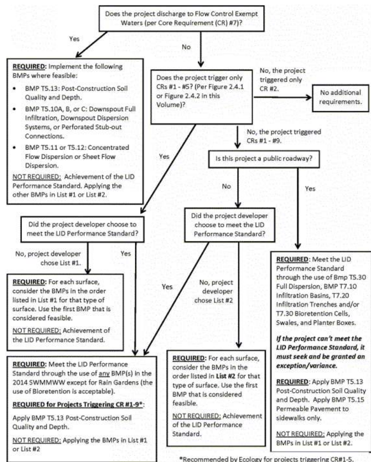
EXHIBIT 4-2 Flow Chart Determining Core Requirement #5 Requirements
