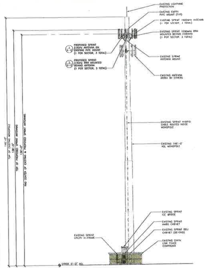
Proposed Elevation View
