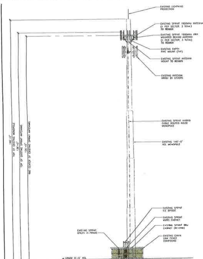
Existing Elevation View
