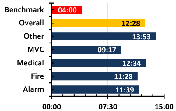
Figure 91: EOFD Travel Time Performance CAD, 2015–2017
