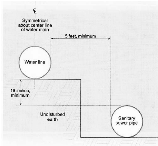
Figure 6-2 Required Separation Between Water Lines and Sanitary Sewers, Unusual Conditions Parallel Construction
