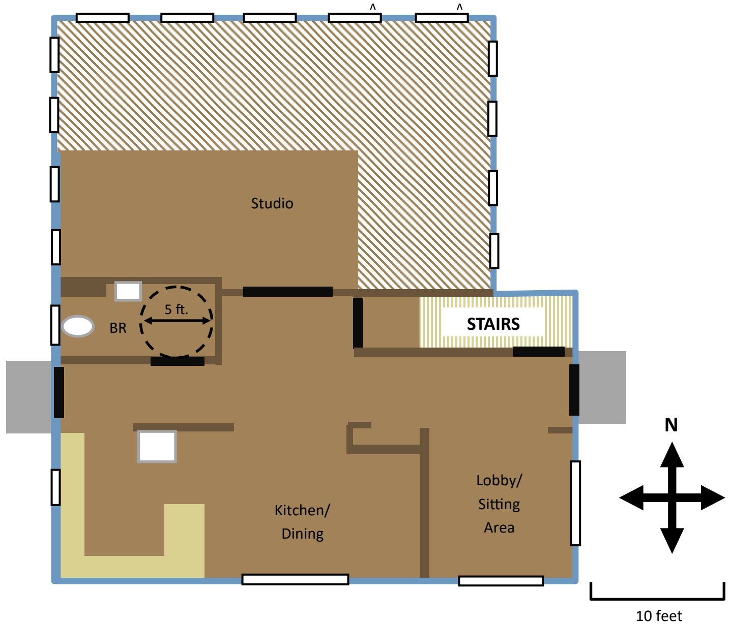
Proposed Interior Building Layout (First Floor)
