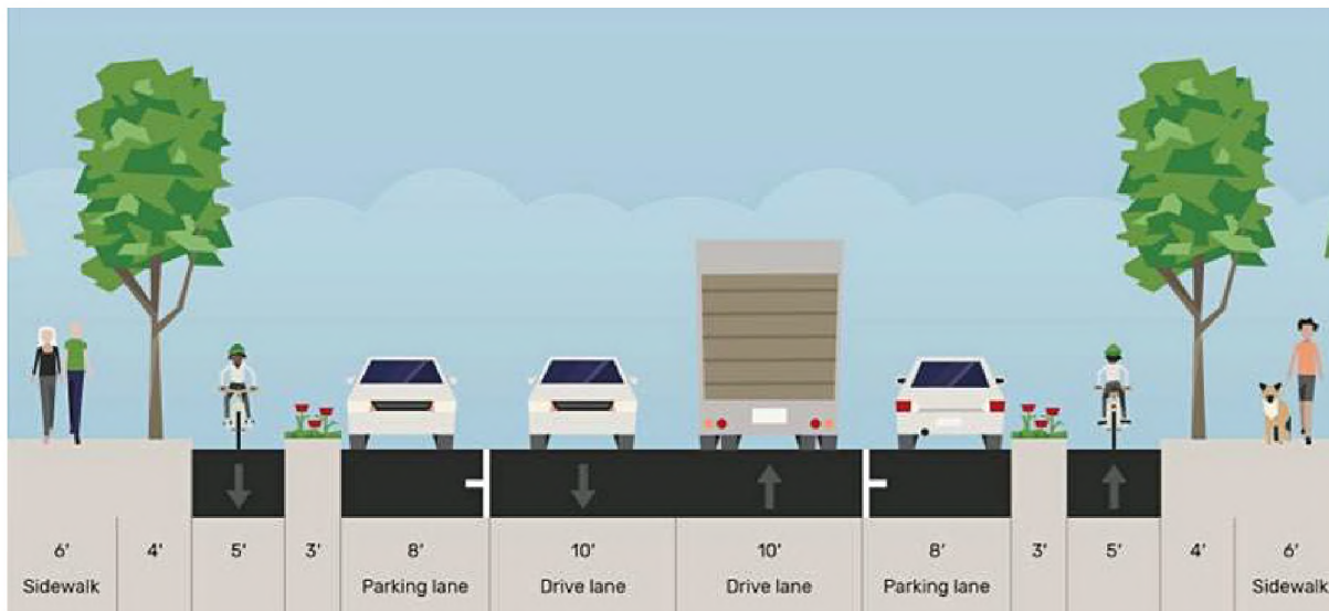
Figure 7-5. Typical street standard option for new essential streets. Some of the first new developments could make use of public funding to meet street requirements.
