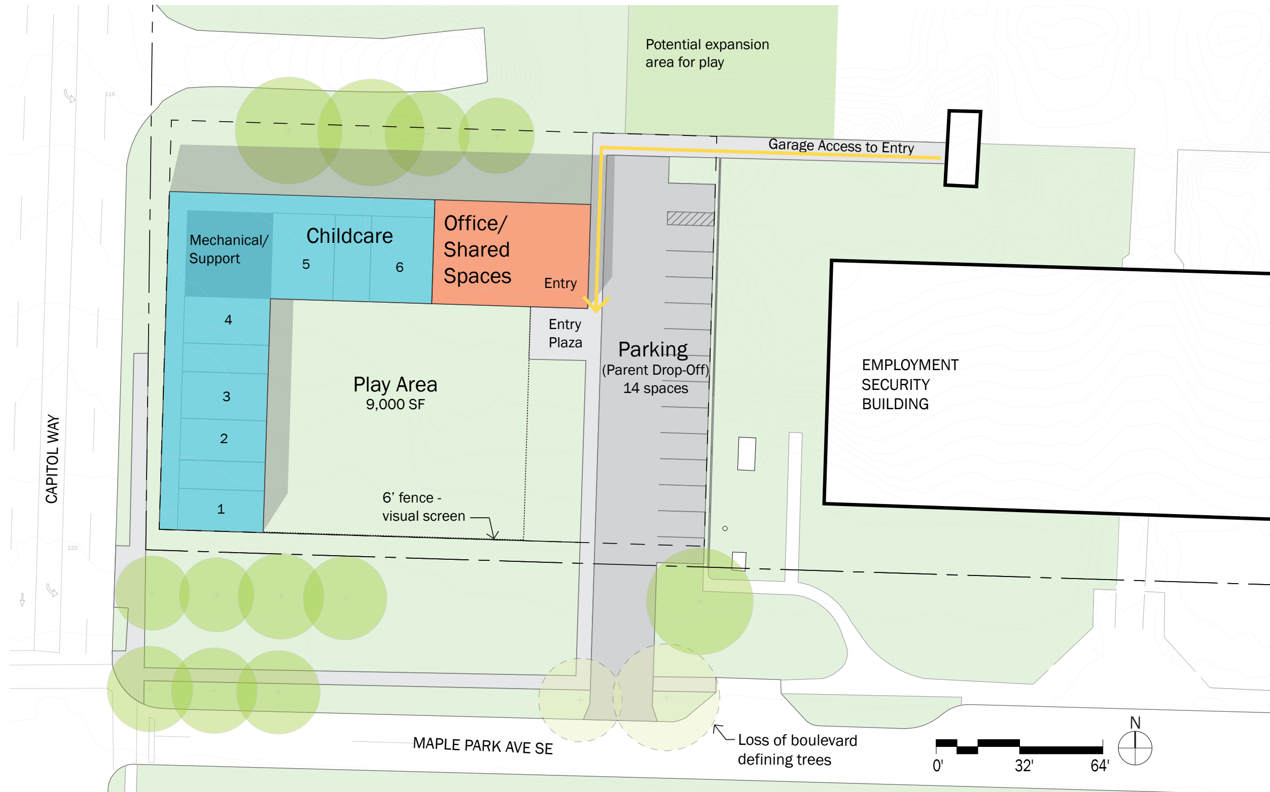
Figure 7-1 Test-to-fit diagram for single story 6 classroom child care
