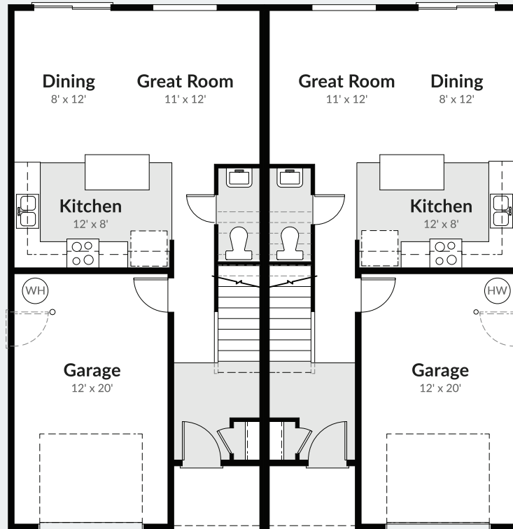
MAIN FLOOR
