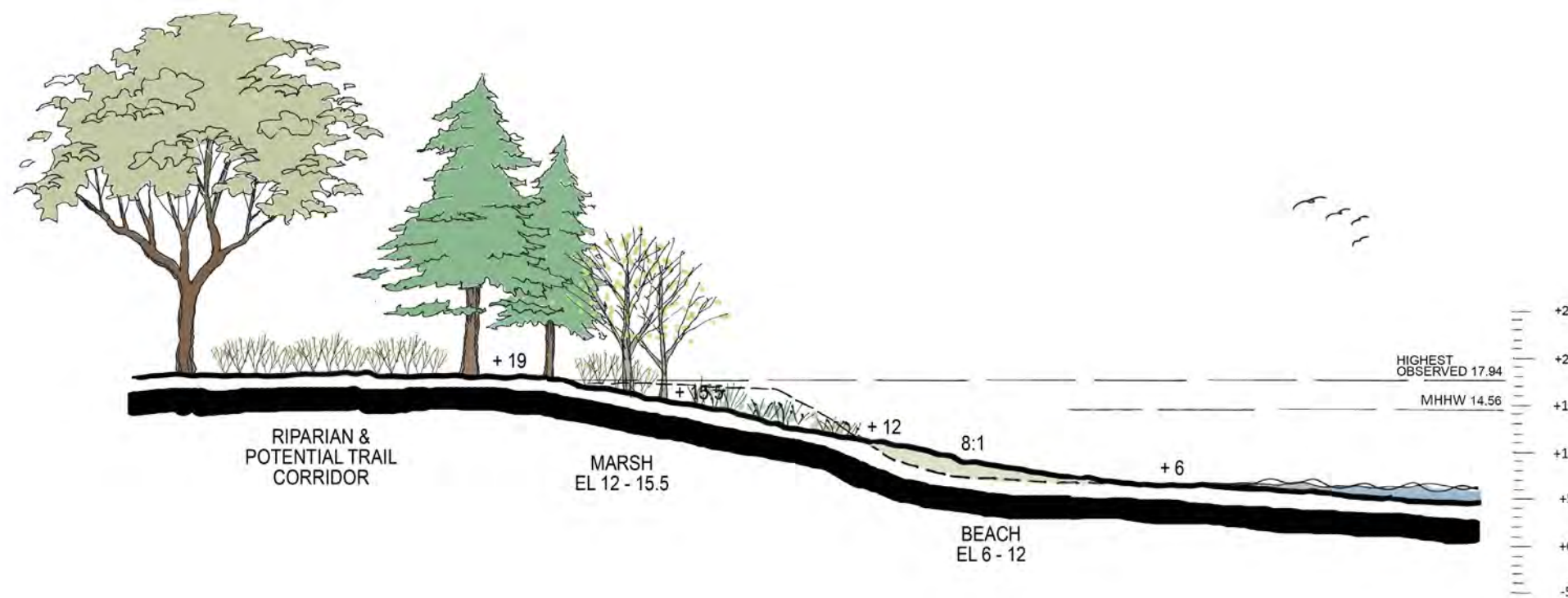
Conceptual Section 11
