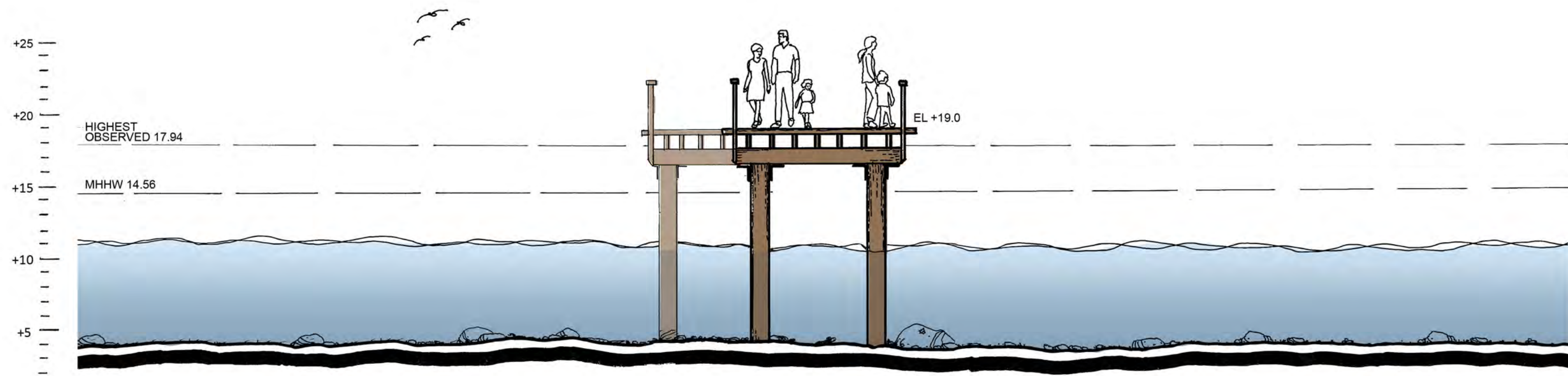
Conceptual Section 2
