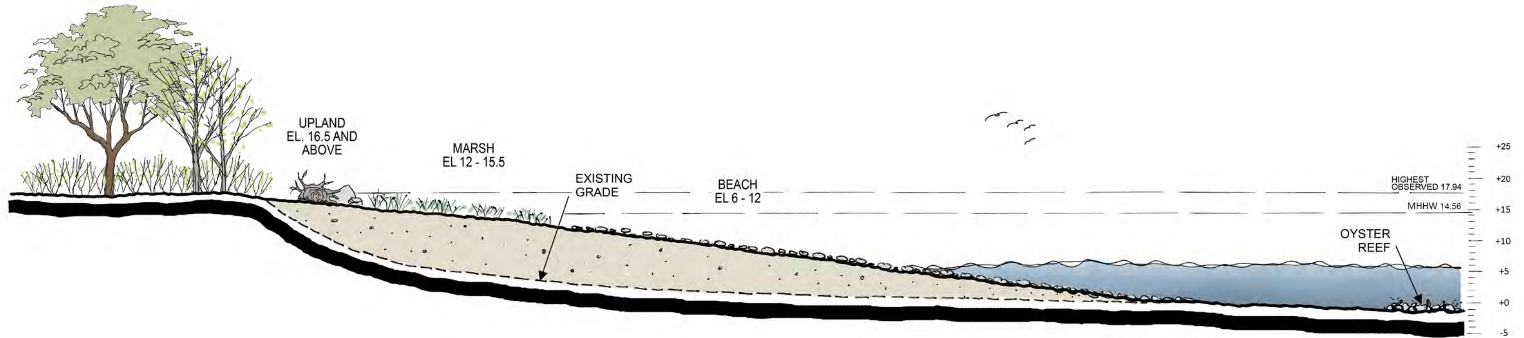
Conceptual Section 17
